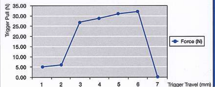
Trigger Pull / Trigger Travel
